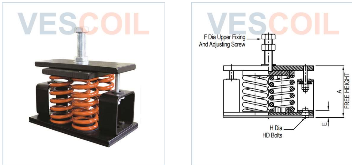
Fig. 9422 | OPEN RESTRAINED SPRING MOUNTINGS - TYPES 25 / 50 - 4 SPRINGS
